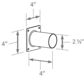
Wall Mount Bracket MPALPRO-WMB
