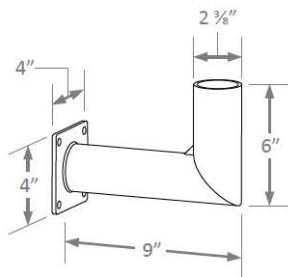
Wall Mount Bracket, 90° MPALPRO-WMB90
